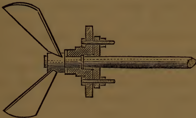
THE EARL OF DUNDONALD'S PROPELLER.
